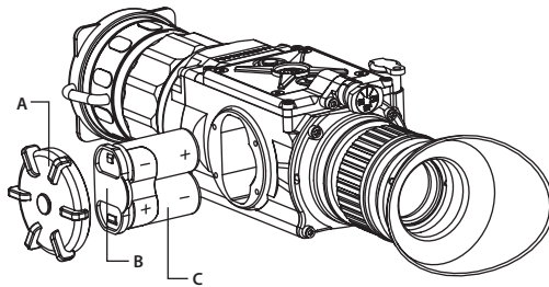
FIGURE 3-1. BATTERY INSTALLATION
