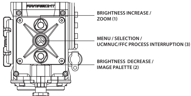
FIGURE 3-17. SETTING BUTTONS
