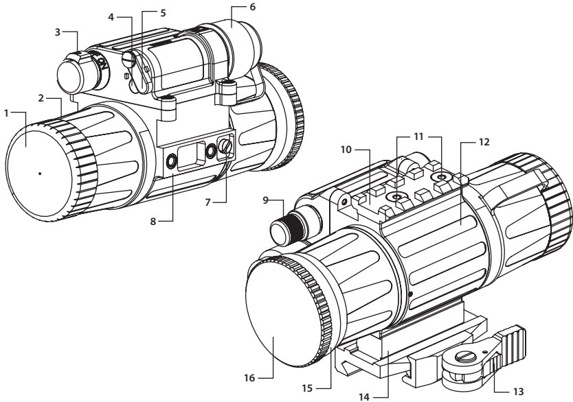
FIGURE 2-2. CO-MINI NIGHT VISION CLIP-ON DEVICE
