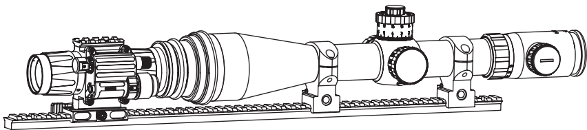
FIGURE 3-6. THE CO-MINI ON A PICATINNY RAIL IN FRONT OF A DAY SCOPE
