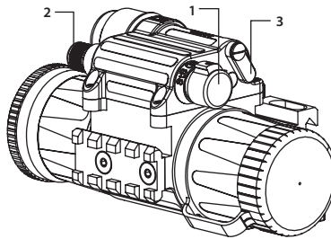
FIGURE 3-17. CO-MINI CONTROLS
