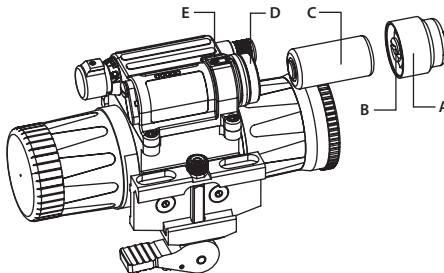
FIGURE 3-1. THE CO-MINI. BATTERY INSTALLATION
