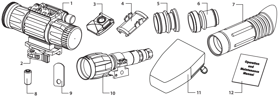
FIGURE 2-3. STANDARD COMPONENTS
