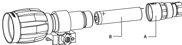
FIGURE 3-3. XLR-IR850 ILLUMINATOR. BATTERY INSTALLATION
